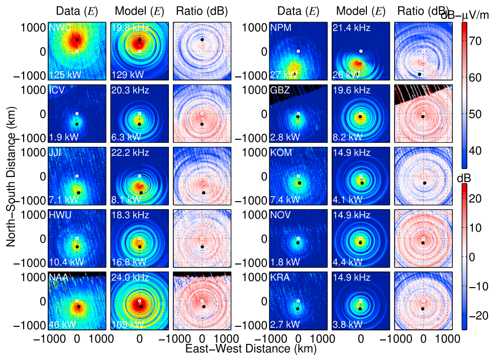
Figure 2. Side by side comparisons of the observed and modeled VLF transmitter signals for each of 10 VLF transmitters (nighttime).
