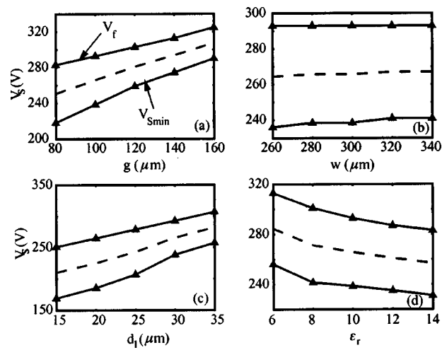
FIG. 3. (a) Firing voltage V_f and the minimum sustaining voltage V_{S\ min} as a function of the sustain electrode gap g . The dashed line shows the mid-margin sustaining voltage V_{S\ m} used for the calculation of UV efficiency; (b) V_f , V_{S\ min} , and V_{S\ m} as a function of the sustain electrode width w ; (c) V_f , V_{S\ min} , and V_{S\ m} as a function of the upper dielectric layer length d_1 ; (d) V_f , V_{S\ min} , and V_{S\ m} as a function of the dielectric constant \epsilon_r .
