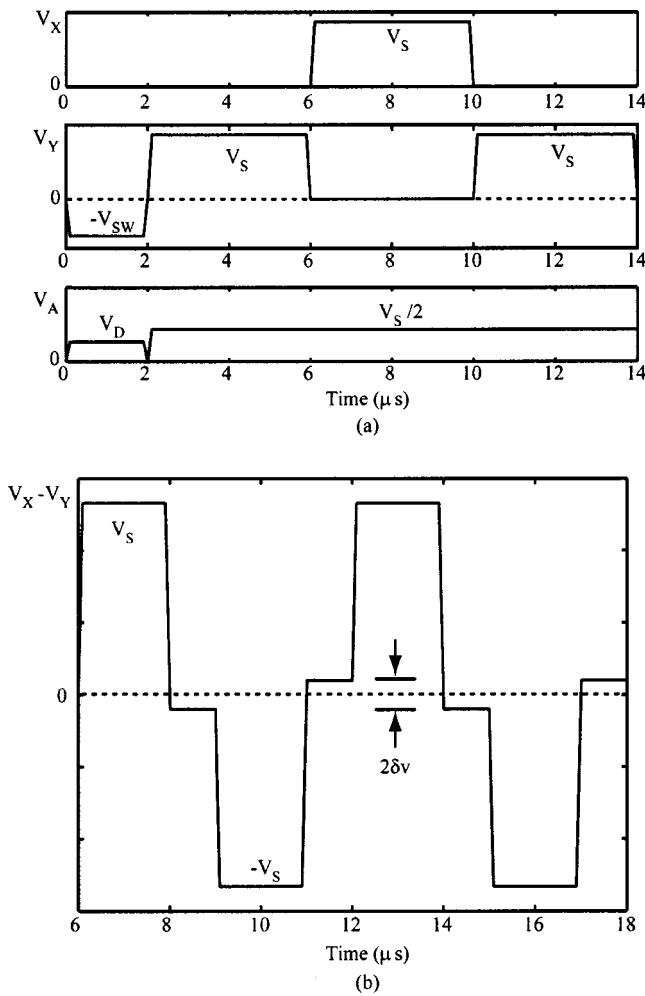
FIG. 2. (a) Driving scheme used in the simulations showing the voltage applied to the X, Y, and A electrodes. Initially, a 2 μs address pulse is applied, followed by a sequence of alternating polarity sustain pulses. The sustaining frequency is 125 kHz. The address electrode is biased to a voltage of V_S/2 during the sustaining phase. (b) The self-erase discharge waveform used in the simulations of Sec. III C. The sustaining frequency is 167 kHz. The 2 μs sustain pulses are followed by a 1 μs assistant pulse. The address electrode is floating during the sustaining phase.
