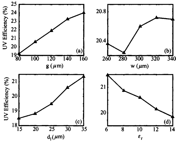
FIG. 5. (a) UV efficiency as a function of the sustain electrode gap g ; (b) UV efficiency as a function of the sustain electrode width w ; (c) UV efficiency as a function of the upper dielectric layer length d_1 ; (d) UV efficiency as a function of the dielectric constant \epsilon_r .
