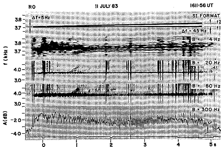
Fig. 7. A two-frequency Siple transmitting experiment in which the frequency difference between two signals of equal strength was varied linearly with time from 5 to 45 Hz, as shown in the top panel. The received spectra, analyzed with varying filter bandwidths, are shown on the next three panels. The bottom panel shows the received amplitude in a 300 Hz band.
