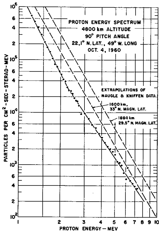
FIGURE 5. Measurements by Bame, Connor, Hill, and Holly using an electronic proton spectrometer in the inner radiation belt.
