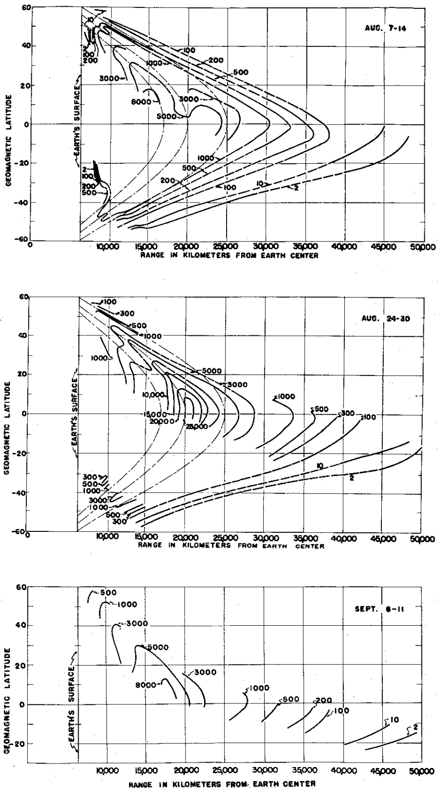
FIGURE 7. Contours of constant counting rate for energetic electrons in the outer radiation belt obtained with the earth satellite Explorer VI.
