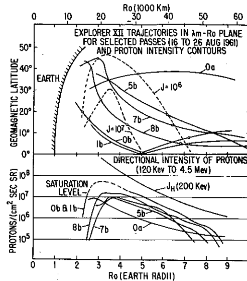
FIGURE 3. Measurement by Davis of the low energy trapped protons on a number of different orbits of the Explorer XII satellite.
