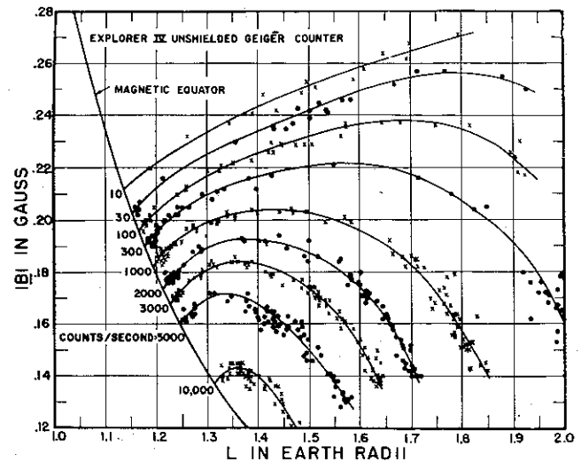
FIGURE 1. A systemization of the intensities of particles in the inner radiation belt.
