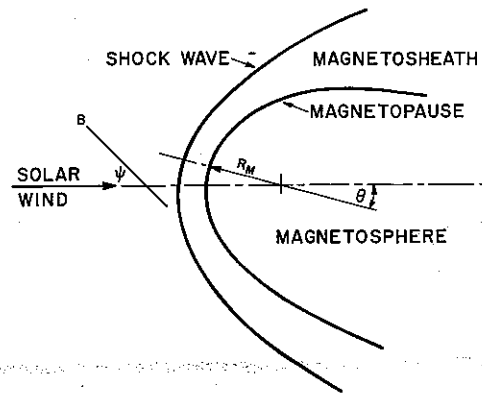
FIGURE 1 Sketch illustrating the interaction of the solar wind with the geomagnetic field [Dessler and Fejer, 1963].
